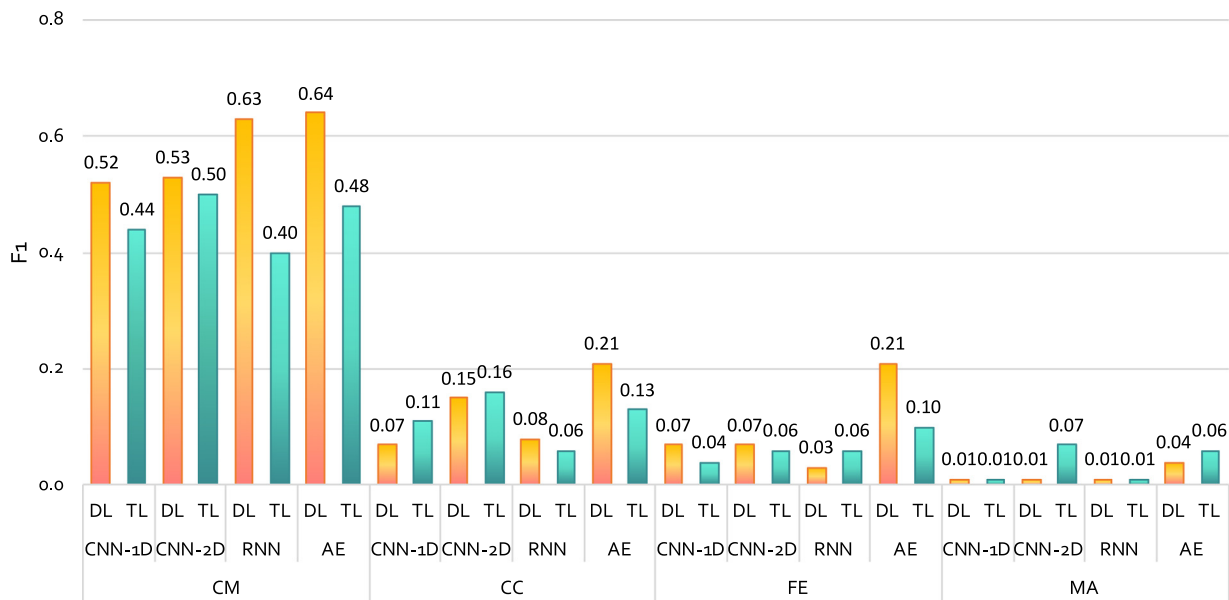
Fig. 12. Comparison of performance of the deep learning models between direct-learning (DL) and transfer-learning (TL) settings.
